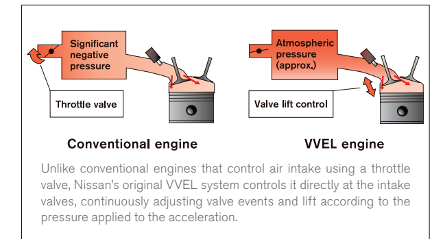
VVEL system
